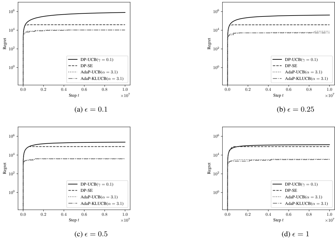
Figure 7: Evolution of regret over time for DP-UCB, DP-SE, AdaP-UCB, and AdaP-KLUCB under C_4 for different values of the privacy budget \epsilon . AdaP-KLUCB achieves the lowest regret.
