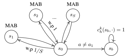
Figure 1: Lower bound construction for non-fresh randomness.
